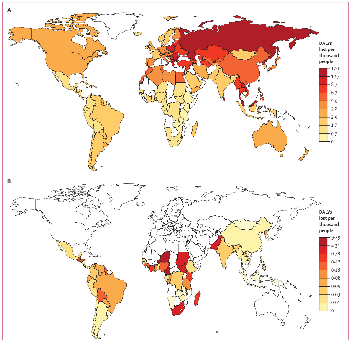
Figure 2: Additional health burden from pollinator removal
